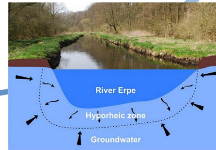
surfacewater - groundwater
