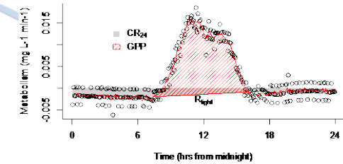
stream metabolism
